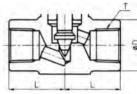
RF : Connection
