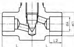
PSW : Connection
