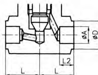
PSW : Connection
