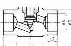
PSW : Connection
