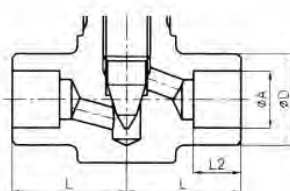
PSW : Connection
